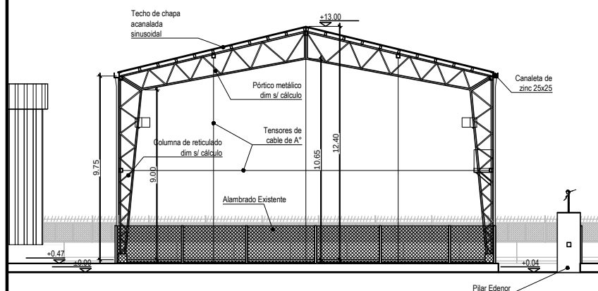
VISTA FRONTAL
