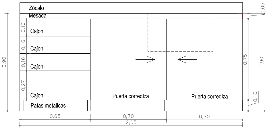
VISTA FRONTAL
